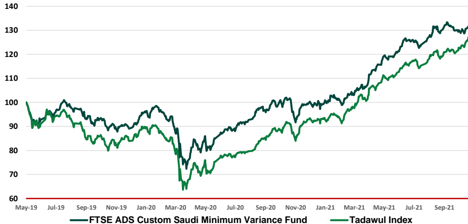
Comparison between FTSE ADS Saudi Minimum Variance Fund and Tadawul Index May 2019 to October 2021 (Rebase to 100)
